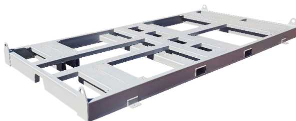
Painted Fork Accessible Skid Frame
